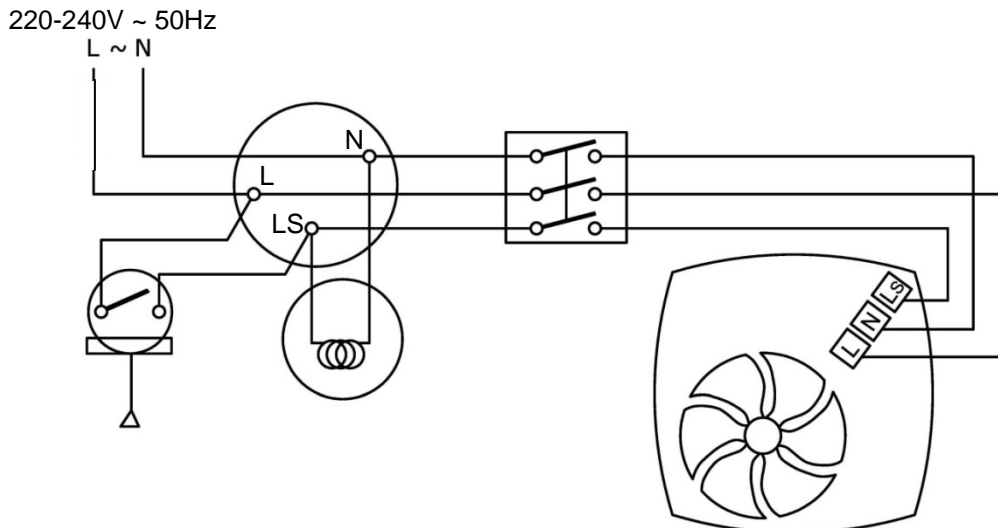
Fig.3: MONS100T/100PIR/125T/150T/100HT/125HT/150HT
