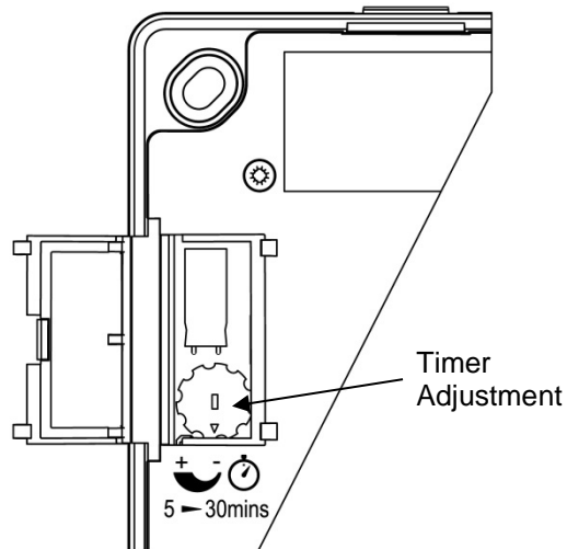
FIG. 5: PIR TIMER
