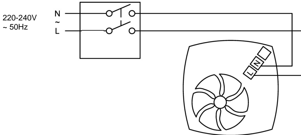
Fig.1: MONS100S/125S/150S/100PIR/100PC
